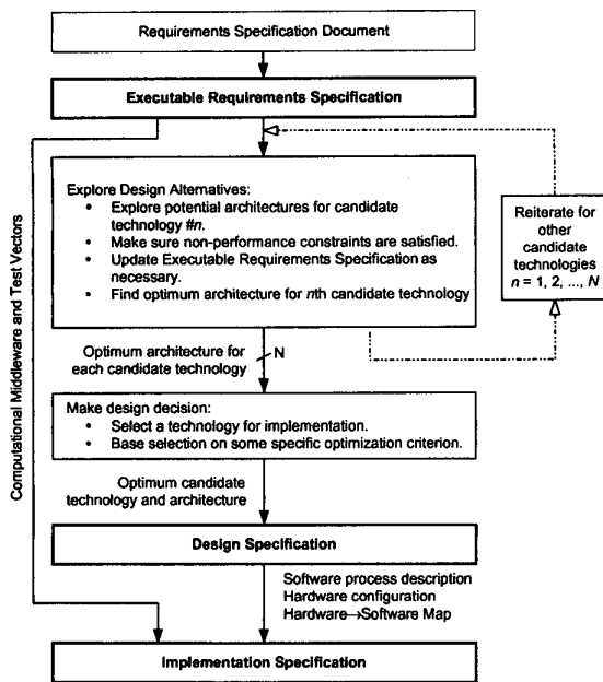
Figure 4. Simplified view of new MAGIC SDM.
